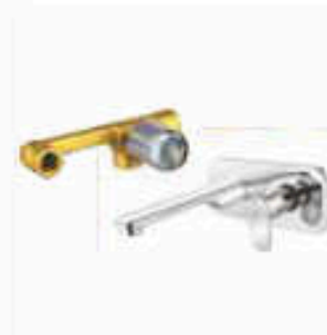
S/L Basin mixer wall mounted exposed parts (35mm) Upper Part 123301 3348/- Conc. Part 180208 3308/-
