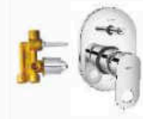
Upper part for S/L concealed diverter 3 Inlet Compatible with 180006 Upper Part 142005 1848/-
